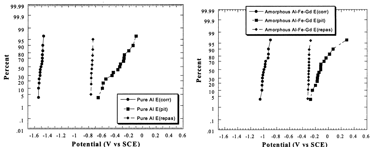
Fig. 4. (a) Cumulative probability plot of E_{\text{corr}} , E_{\text{pit}} , and E_{\text{rep}} for high purity polycrystalline Al mb electrode (surface area of 10^{-4} \text{ cm}^2 ) in deaerated 0.6 M NaCl. (b) Cumulative probability plot of E_{\text{corr}} , E_{\text{pit}} , and E_{\text{rep}} for \text{Al}_{90}\text{Fe}_5\text{Gd}_5 mb electrode (surface area of 10^{-4} \text{ cm}^2 ) in deaerated 0.6 M NaCl.
