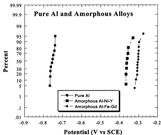
Fig. 5. Cumulative probability plot of E_{\text{rep}} for pure Al and amorphous alloy mb electrodes (surface area of 10^{-4} \text{ cm}^2 ) in deaerated 0.6 M NaCl showing the improved pit corrosion resistance of both amorphous alloys.
