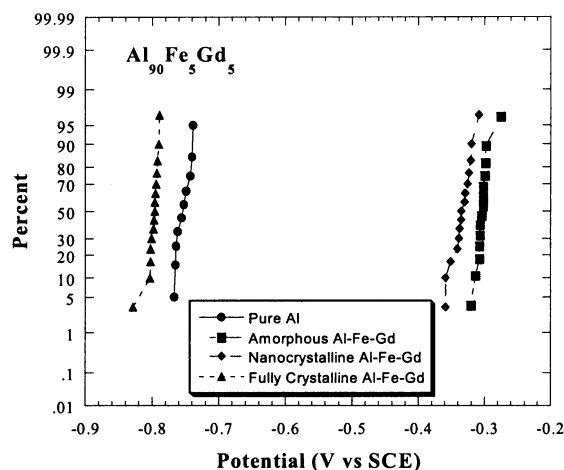
Fig. 6. Cumulative probability plot of E_{\text{rep}} values for amorphous, nanocrystalline, and crystalline \text{Al}_{90}\text{Fe}_5\text{Gd}_5 mb electrodes (surface area of 10^{-4} \text{ cm}^2 ) in comparison to pure Al in deaerated 0.6 M NaCl.
